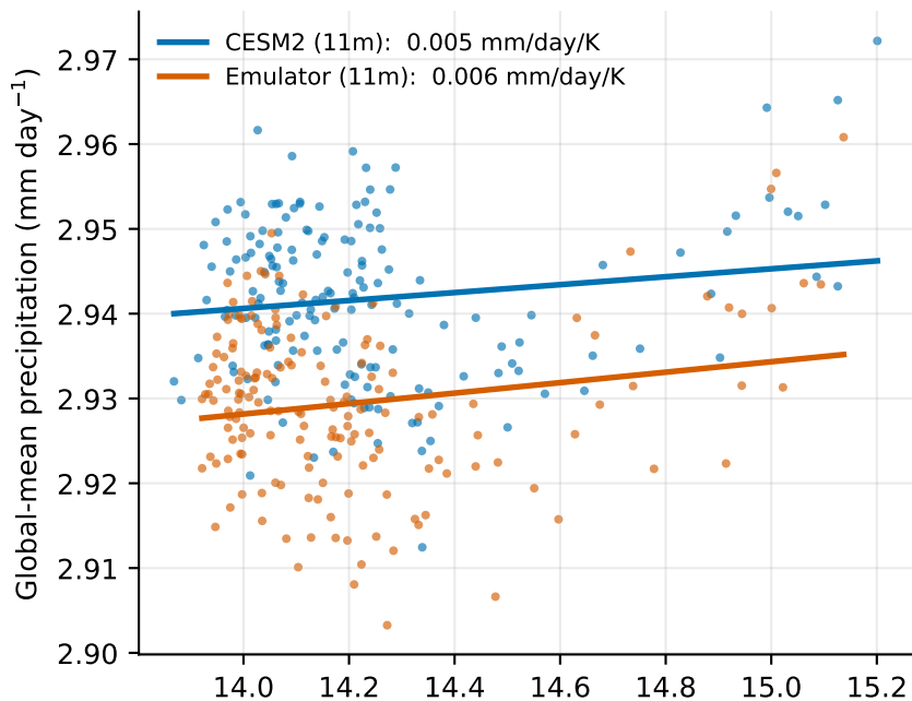
(c) Aerosol-only
