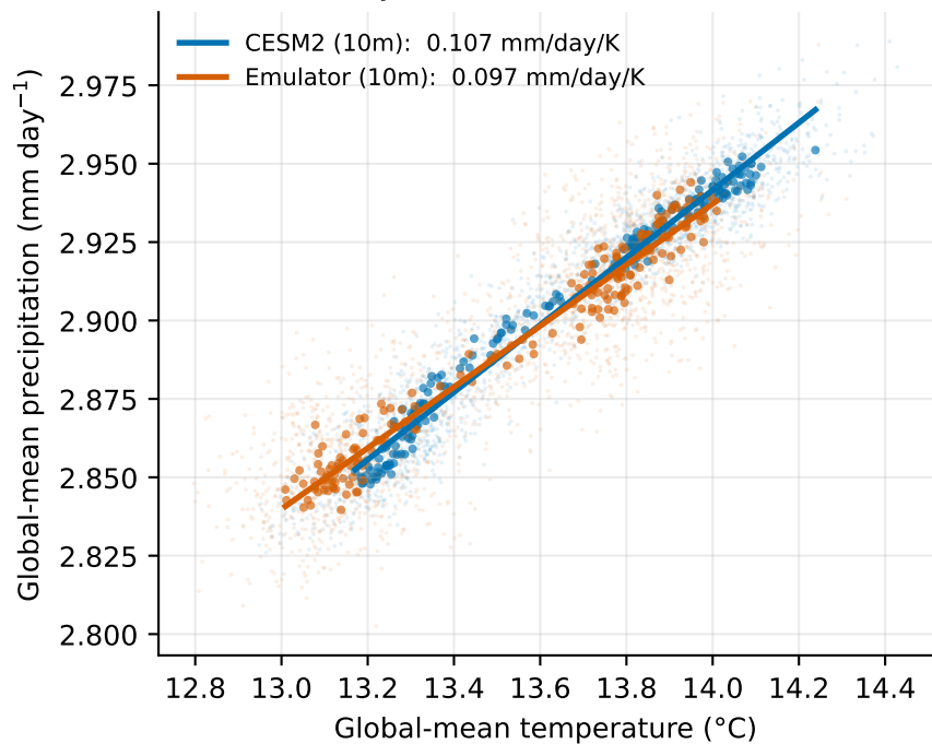
(c) Aerosol-only
