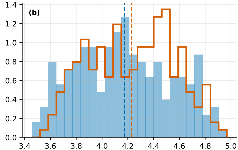
Greenhouse-gas-only (GHG) (2031–2050) \Delta\text{mean} -0.066 , sd ratio 1.03
