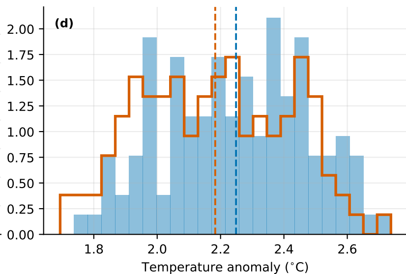
Greenhouse-gas-only (GHG) (2031–2050) \Delta\text{mean} -0.066 , sd ratio 1.03
