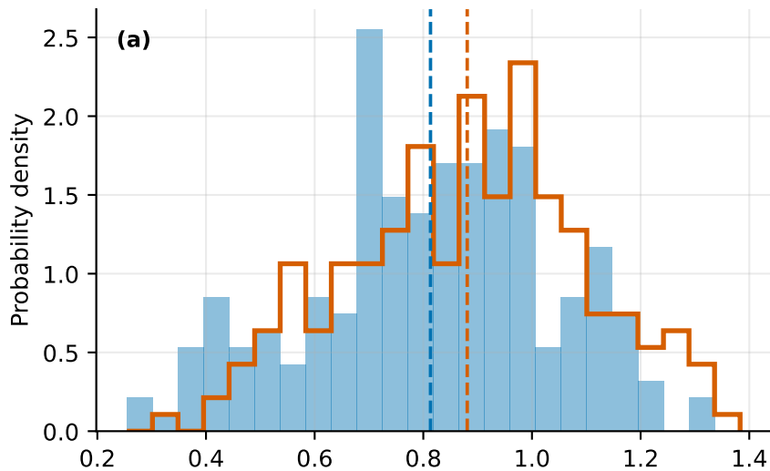
Aerosol-only (AAER) (2031–2050) \Delta\text{mean} -0.002 , sd ratio 0.92
