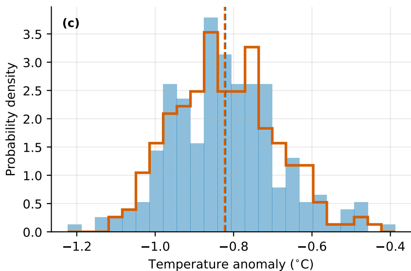
Aerosol-only (AAER) (2031–2050) \Delta\text{mean} -0.002 , sd ratio 0.92
