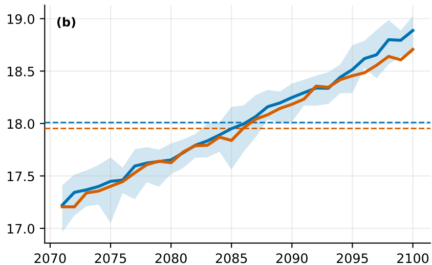
Greenhouse-gas-only (GHG) offset -0.172, CESM2 member range 2× wider
