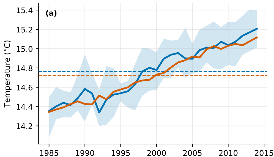
Aerosol-only (AAER) offset -0.127, CESM2 member range 4× wider
