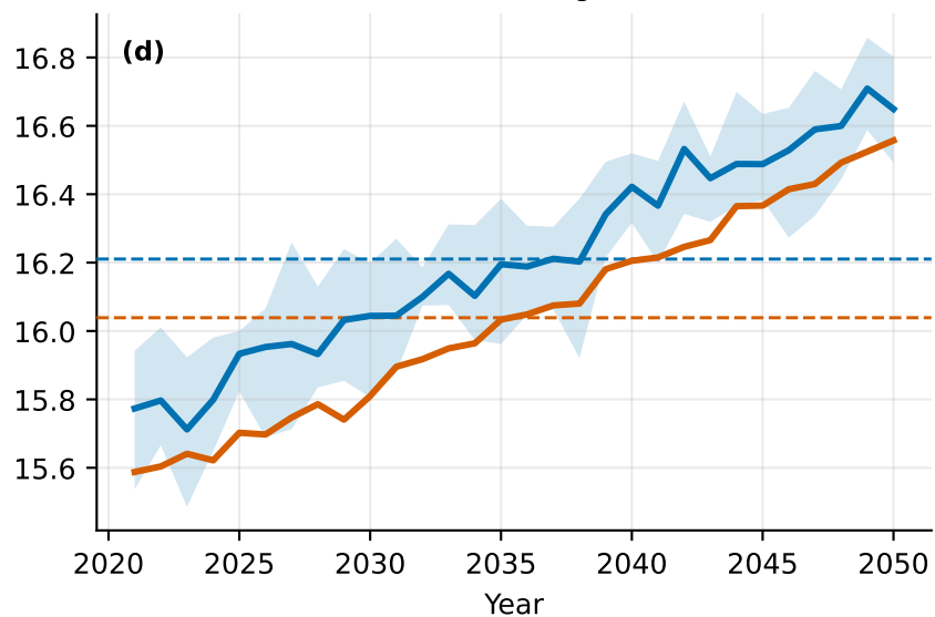
Greenhouse-gas-only (GHG) offset -0.172, CESM2 member range 2× wider
