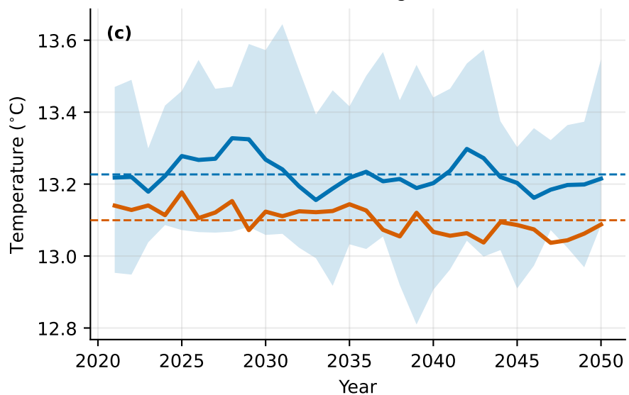
Aerosol-only (AAER) offset -0.127, CESM2 member range 4× wider
