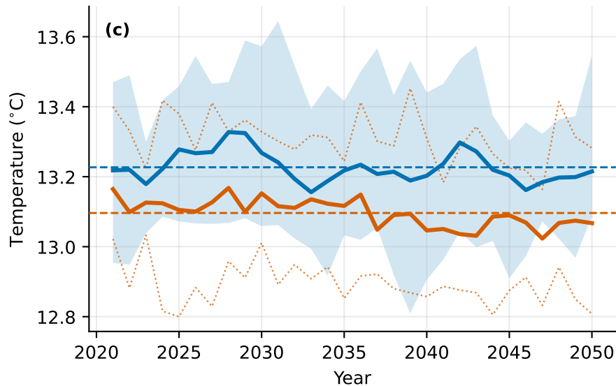
Aerosol-only (AAER) offset -0.131, CESM2 member range 3× wider
