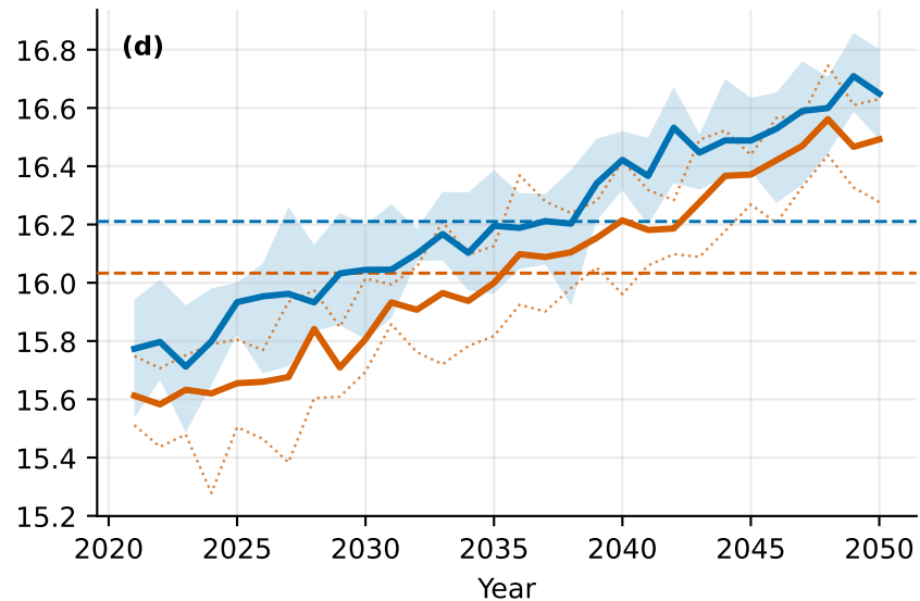
Greenhouse-gas-only (GHG) offset -0.177, CESM2 member range 2× wider
