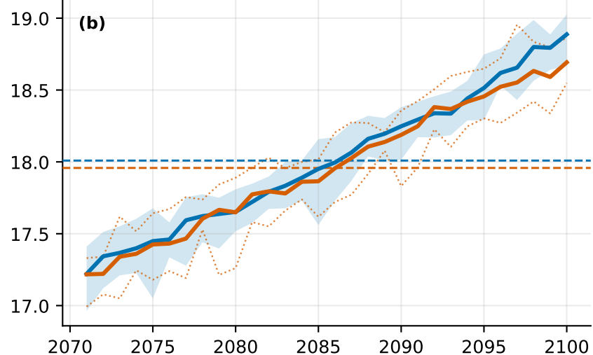
Greenhouse-gas-only (GHG) offset -0.177, CESM2 member range 2× wider
