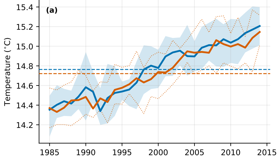
Aerosol-only (AAER) offset -0.131, CESM2 member range 3× wider
