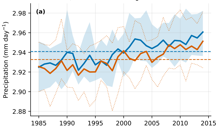
Aerosol-only (AAER) offset -0.005, CESM2 member range 8× wider
