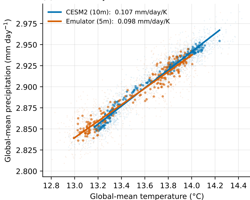
(c) Aerosol-only
