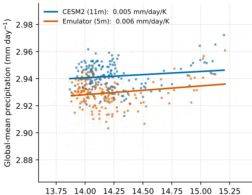
(c) Aerosol-only
