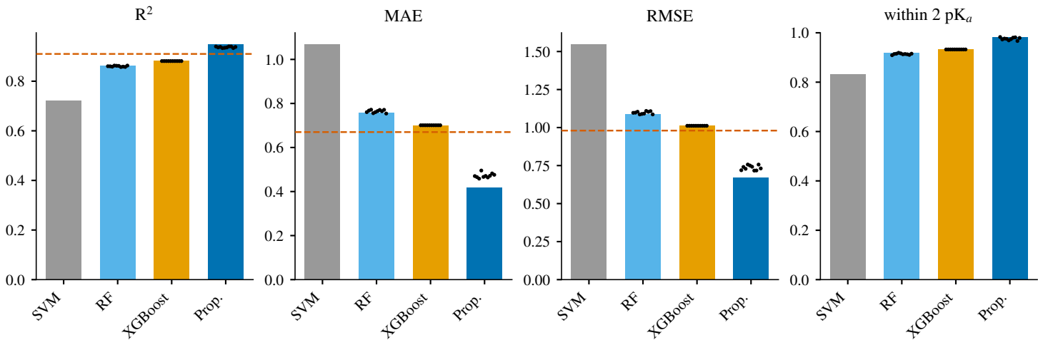
pKa_Basic: untuned baselines vs proposed (bars: ensemble; dots: single seeds; dashed: published benchmark)
