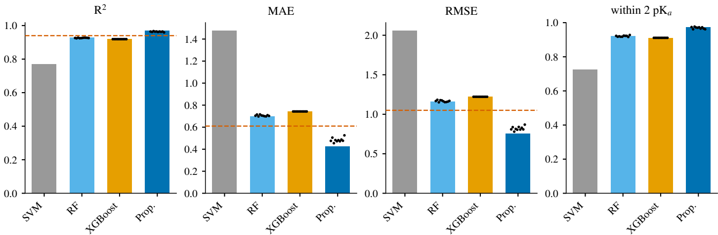
pKa_Acidic: untuned baselines vs proposed (bars: ensemble; dots: single seeds; dashed: published benchmark)
