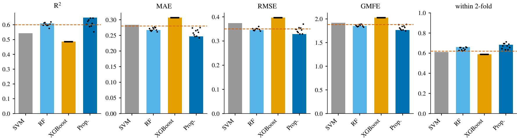
VDss: untuned baselines vs proposed (bars: ensemble; dots: single seeds; dashed: published benchmark)
