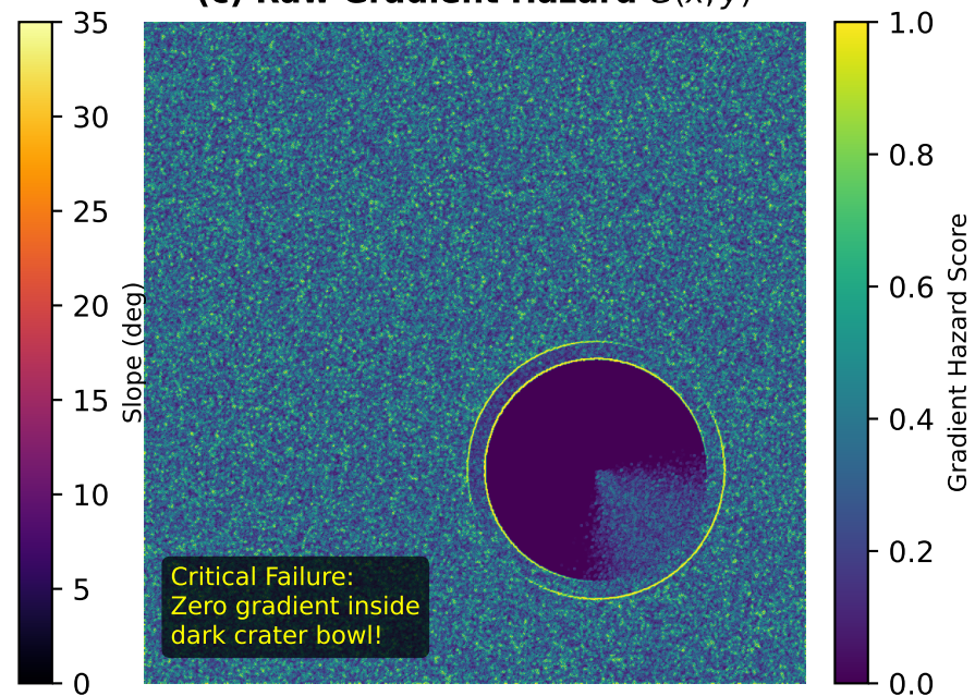
(c) Raw Gradient Hazard G(x, y)
