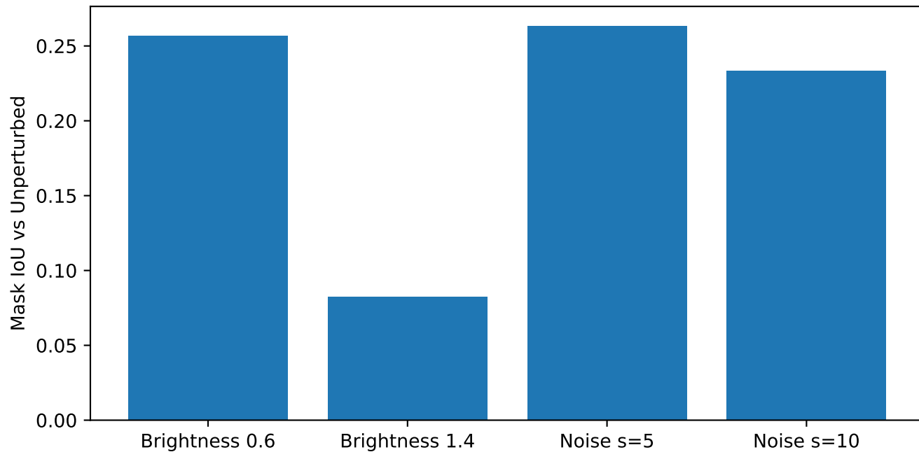
Robustness of Full Pipeline (Config D)
