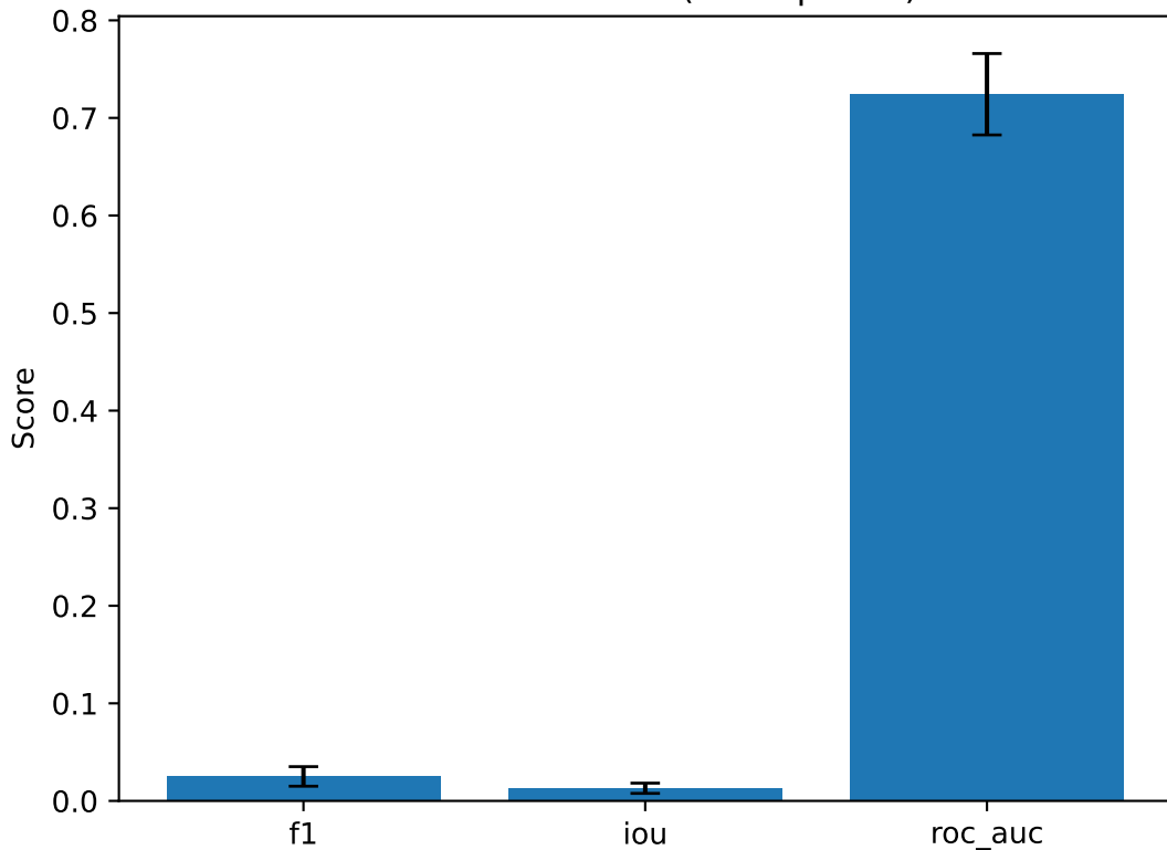
TEST Set Metrics (Full Pipeline)
