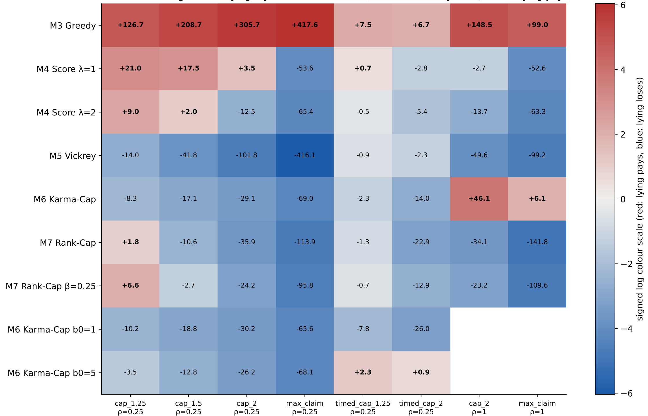
E10 — Unilateral gain from lying, by mechanism and lie (numbers = utility units; bold = lying pays)
