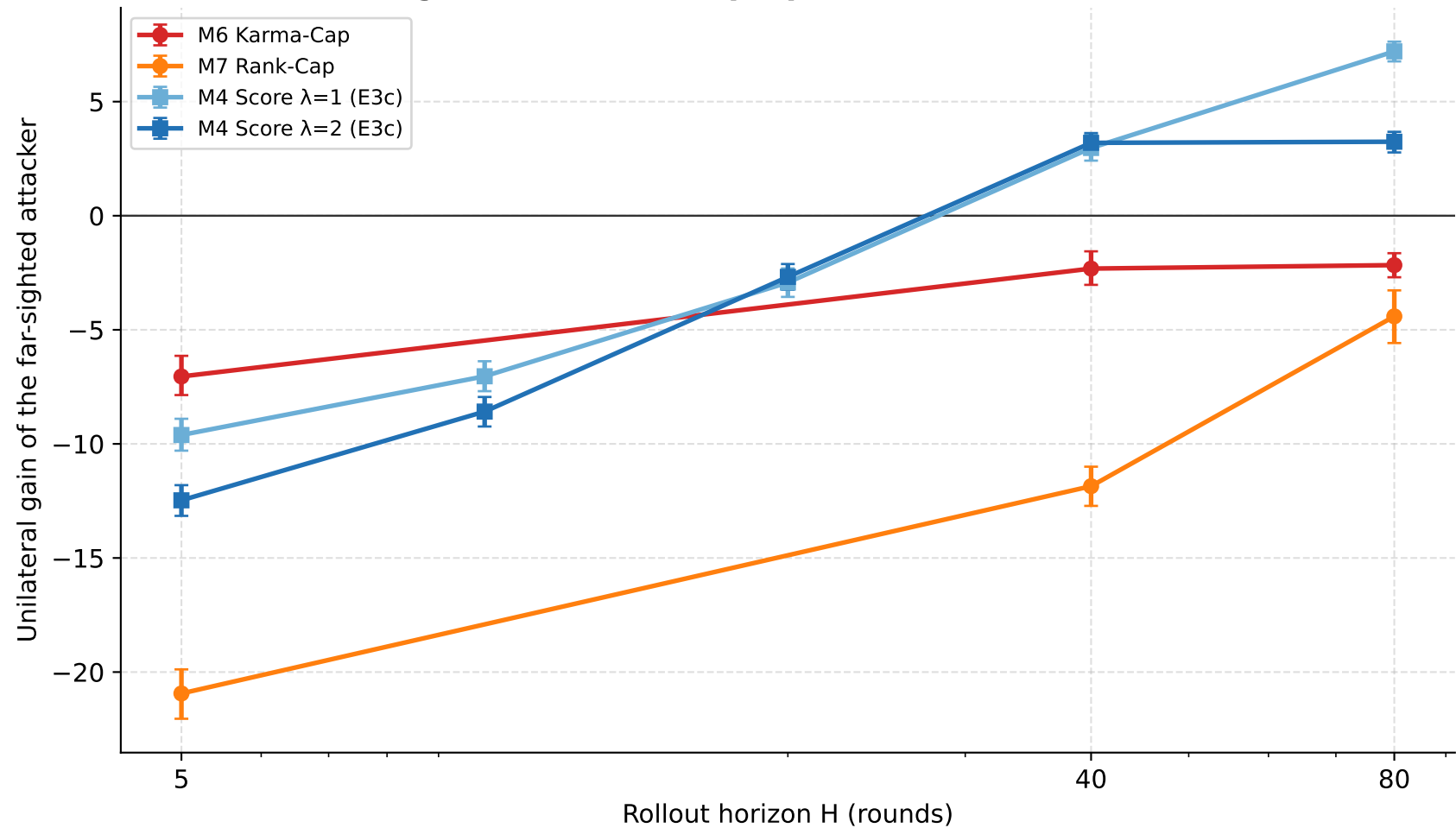
E11 — Far-sighted attacker vs proposed mechanisms (n=10, T=300)
