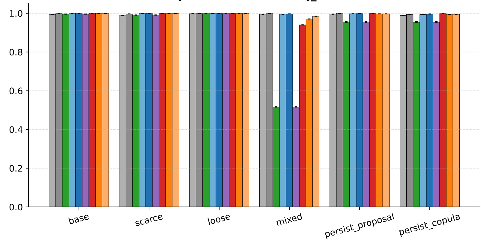
Starvation rate SR_Δ
