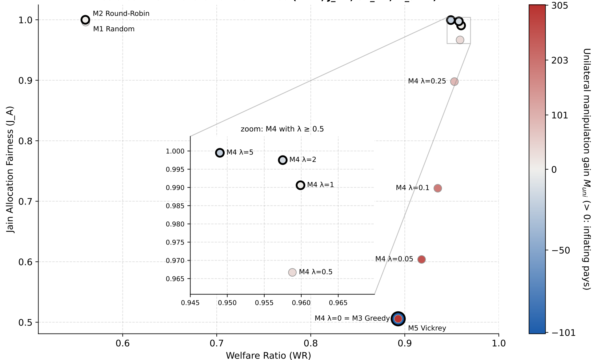
E2 — Fairness / Efficiency / Manipulation Frontier ( p = 0.25 , capped exaggeration c = 2 ) bold outline = Pareto non-dominated (WR \uparrow , J_A \uparrow , SR_ \Delta \downarrow , M_uni \downarrow )
