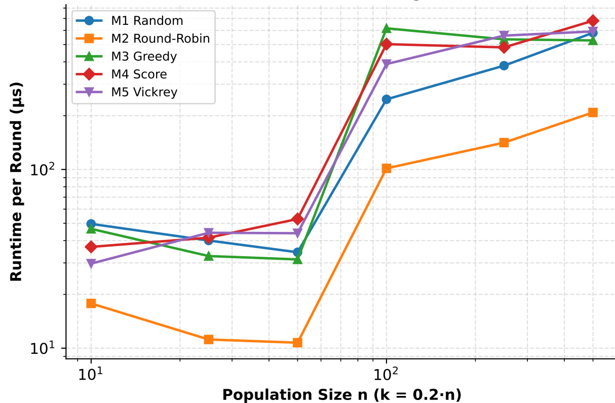
Runtime Scaling
