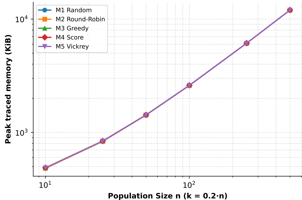
Peak Memory (tracemalloc)
