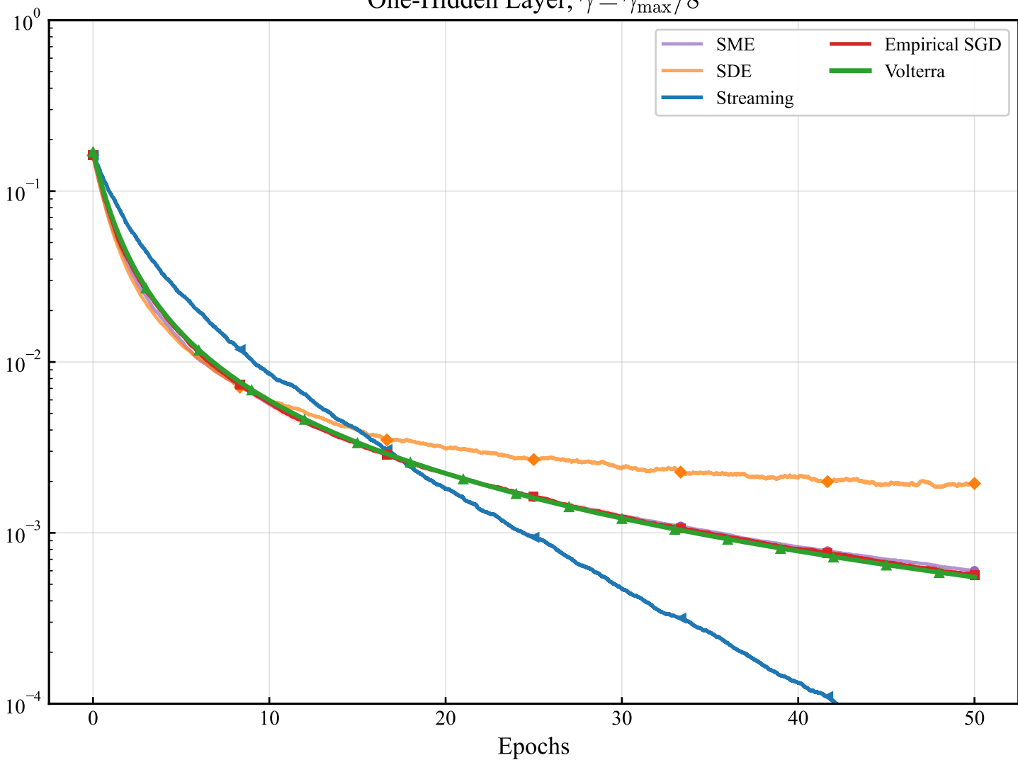
One-Hidden Layer, \gamma = \gamma_{\max}/8
