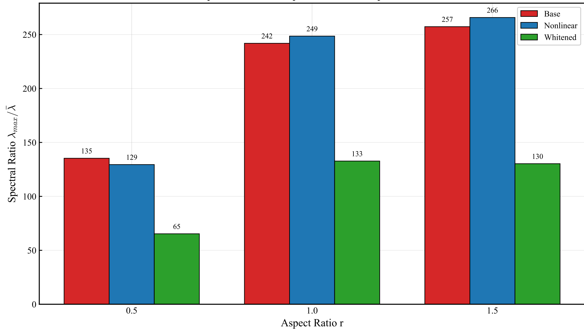
Spectral Ratio Comparison Across Experiments
