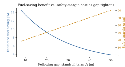
Figure 4: Estimated fuel-saving benefit and safety margin as functions of the commanded following gap, at the default fleet size and speed.
