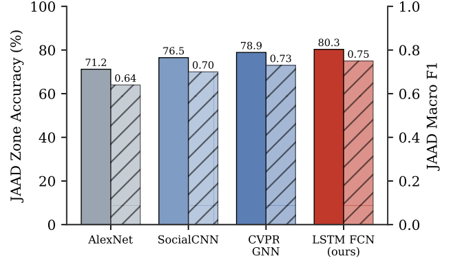
Fig. 2. Template comparison of intersection estimation performance on JAAD. Left axis / solid bars: zone accuracy; right axis / hatched bars: macro F1.
