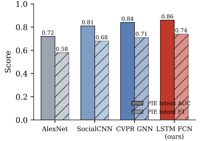
Fig. 3. Template comparison of intention tracking performance on PIE. Solid bars: AUC; hatched bars: F1 at a 0.5 probability threshold.
