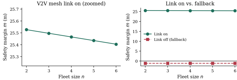
Figure 3: Safety margin m against fleet size n , evaluated at the demonstrator’s default following gap and road speed, with the V2V mesh link on versus the onboard-perception-only fallback. Values are computed from the model of Eqs. (2), (4) and (5) using representative design-budget latencies (Table 2); the crossing of the fallback curve toward the zero-margin line is the qualitative behaviour of interest, not a field-measured bound.
