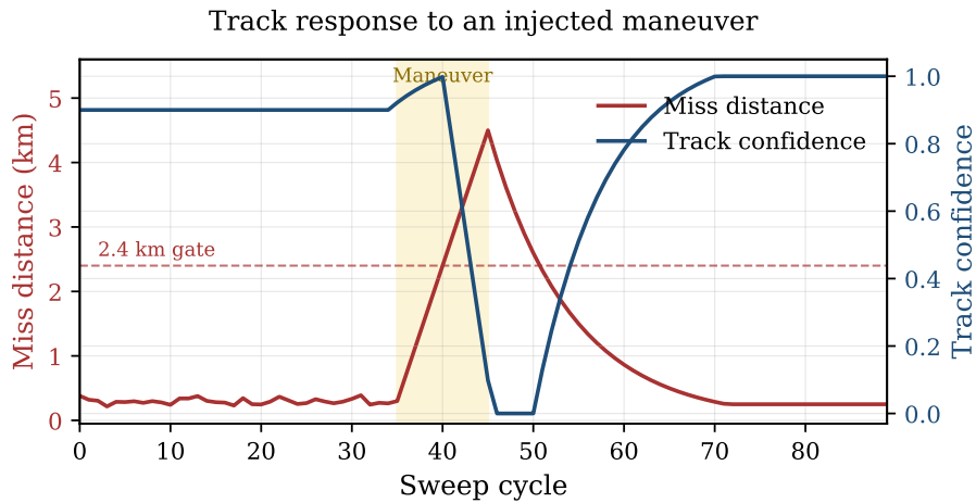
Figure 2: Miss distance between predicted and detected position (left axis) and track confidence (right axis) across an injected maneuver window, illustrating the gate-exceedance → confidence-decay → reconvergence pattern described in Section 5.3. Values are representative of the demonstrator’s qualitative behaviour rather than a specific logged run.
