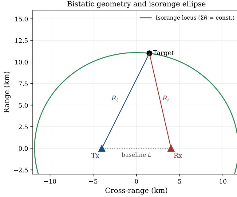
Figure 3: Illustrative bistatic geometry: transmitter (Tx) and receiver (Rx) separated by baseline L , a target at range legs R_t and R_r , and the isobistatic-range (isorange) ellipse with foci at Tx and Rx corresponding to the current bistatic range sum \Sigma R = R_t + R_r (Section 2).
