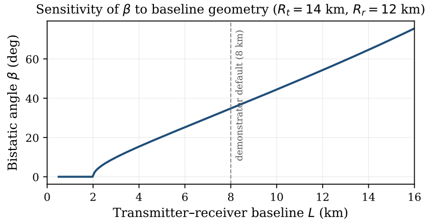
Figure 4: Bistatic angle \beta computed from Eq. 1 as a function of transmitter–receiver baseline L , at fixed representative ranges R_t = 14 km and R_r = 12 km. \beta increases monotonically with baseline separation, consistent with the qualitative sensitivity described in Section 2; the dashed line marks the demonstrator’s 8 km default baseline (Table 1).
