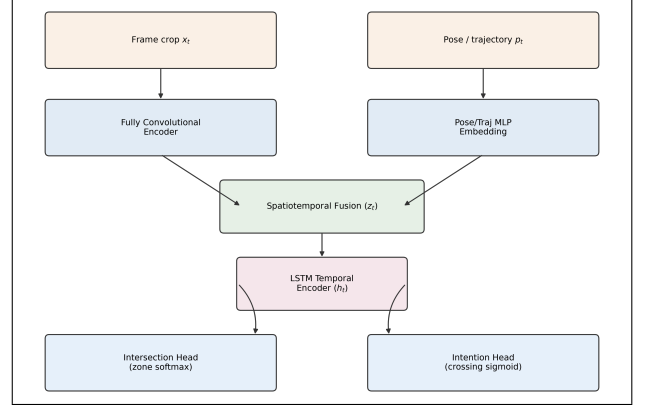
Fig. 1. Overview of the proposed LSTM FCN architecture.
