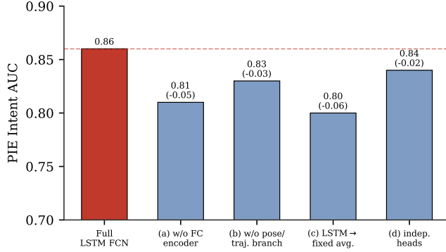
Fig. 4. Template ablation results on PIE intention tracking AUC. The dashed line marks the full model AUC; parenthetical values give \Delta vs. the full model.
