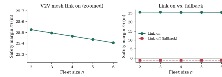
Figure 3: Safety margin m against fleet size n , evaluated at the demonstrator's default following gap and road speed with the V2V mesh link on versus the onboard-perception-only fallback. Values are computed.
