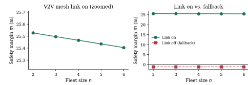
Figure 3: Safety margin m against fleet size n , with the V2V mesh link on versus the onboard-perception-only fallback, evaluated at the demonstrator's default following gap and road speed.
