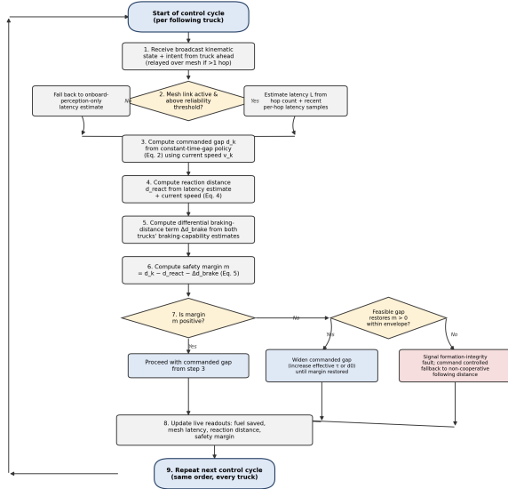
Figure 6: Flowchart of the per-cycle platooning gap-control logic from Appendix B, showing the mesh-link fallback branch (step 2) and the margin-feasibility branch (steps 6–7).
