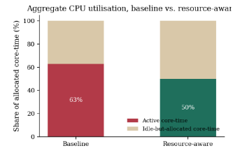
Figure 2: Aggregate share of allocated core-time spent active versus idle-but-allocated, baseline versus resource-aware scheduler, per the utilisation definition of (1).
