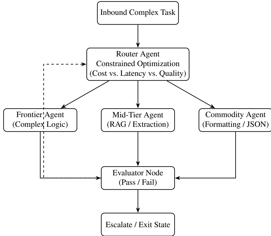
Figure 1: High-level routing architecture. The Router Agent intercepts each execution frame and dynamically dispatches to the frontier, mid-tier, or commodity agent pool based on the constrained optimization solved at runtime. An Evaluator Node closes the loop by scoring outputs for pass/fail escalation (dashed feedback path).
