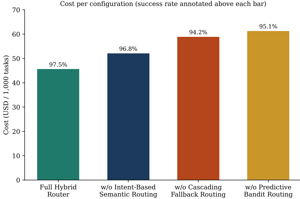
Figure 4: Ablation study results (Table 2). Bars show total run cost per configuration; the annotated percentage above each bar is the corresponding workflow success rate.
