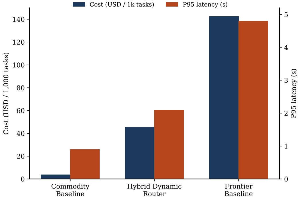
Figure 2: Total run cost and P95 latency across the three evaluated configurations (Table 1). The Hybrid Dynamic Router sits between the two extremes on both axes, but far closer to the commodity baseline than to the frontier baseline.
