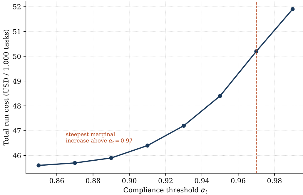
Figure 5: Total run cost as a function of the compliance threshold \alpha_t . Cost increases monotonically and convexly, with the steepest marginal increase observed above \alpha_t = 0.97 .
