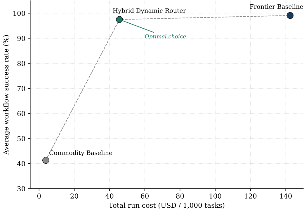
Figure 3: Cost versus accuracy for the three evaluated configurations. The Hybrid Dynamic Router sits close to the frontier baseline’s accuracy while incurring less than one-third of its cost.
