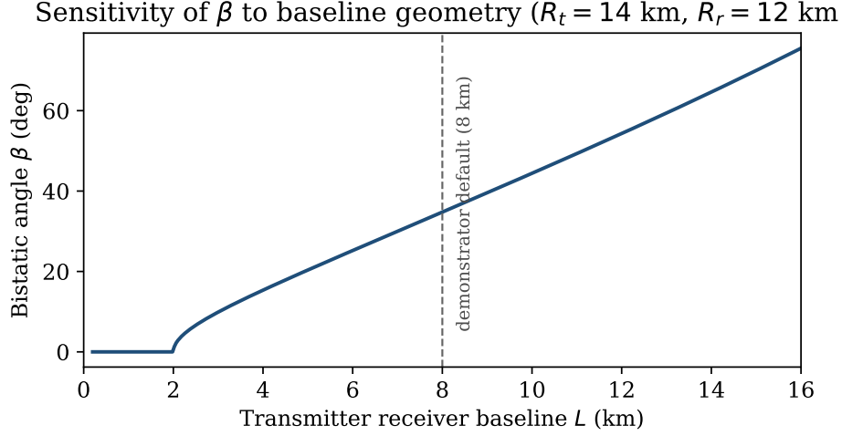
Figure 4: Bistatic angle \beta computed from Equation 1 as a function of transmitter receiver baseline L , at fixed representative ranges R_t = 14 km and R_r = 12 km. \beta increases monotonically with baseline separation, consistent with the qualitative sensitivity described in Section 2; the dashed line marks the demonstrator’s 8 km default baseline (Table 1).
