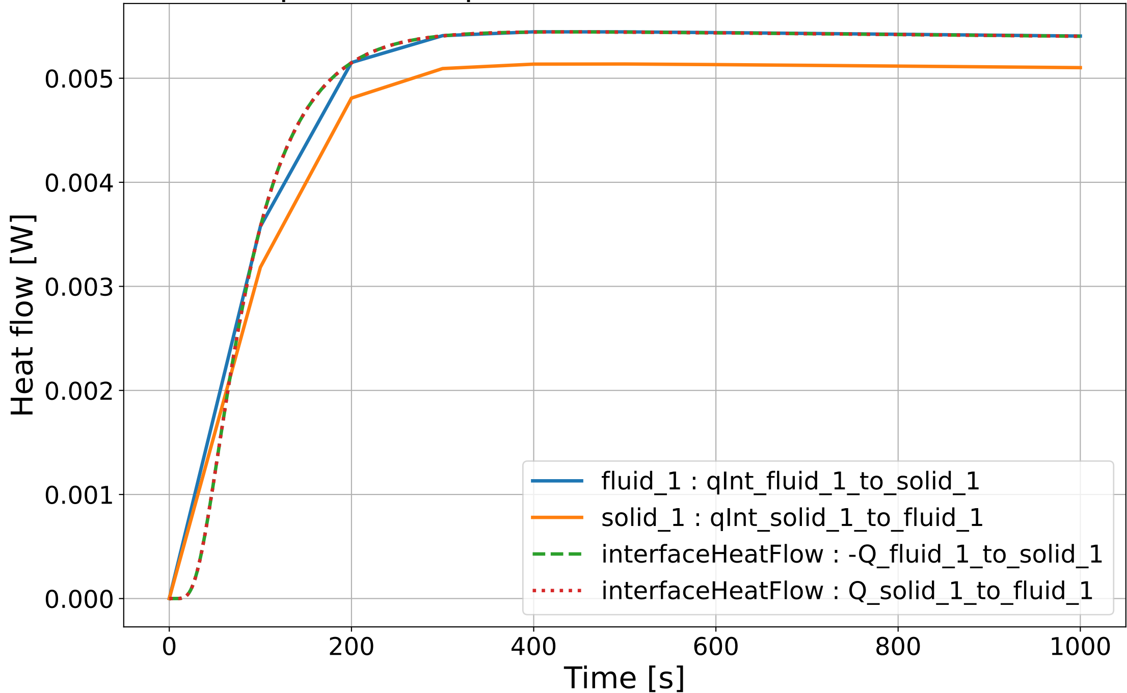
Comparison of qInt and interfaceHeatFlow histories
