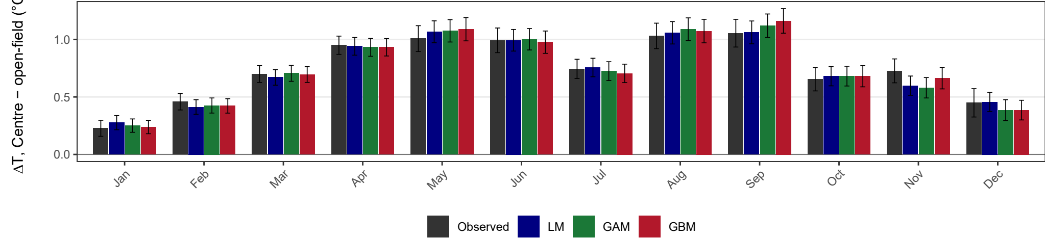
Monthly mean \Delta T : modelled vs observed (held-out test split)
