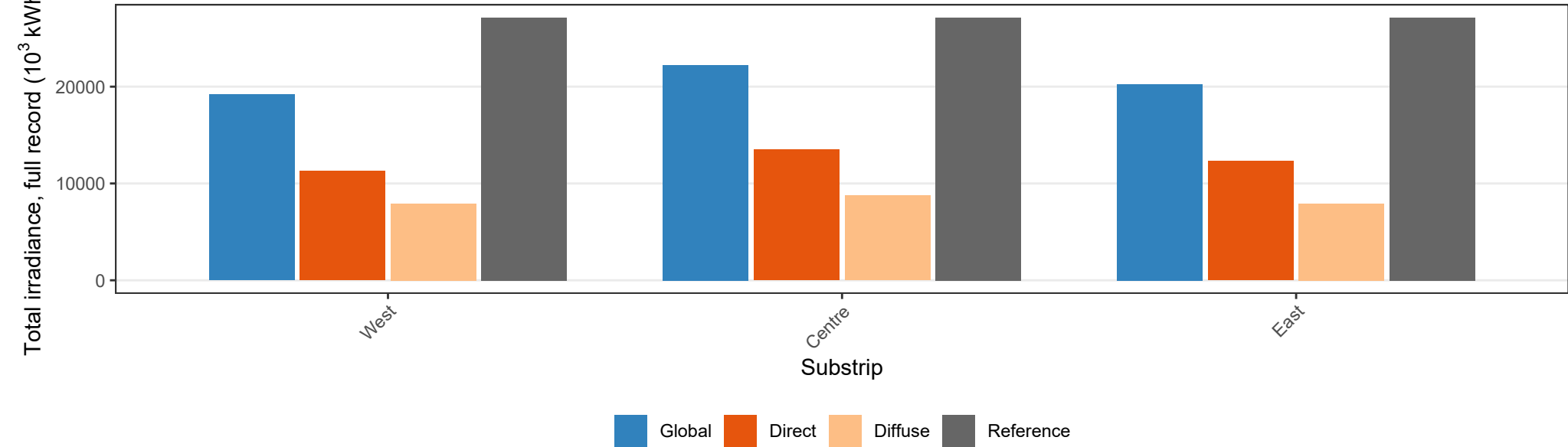
Cumulative radiation budget by substrip and component
