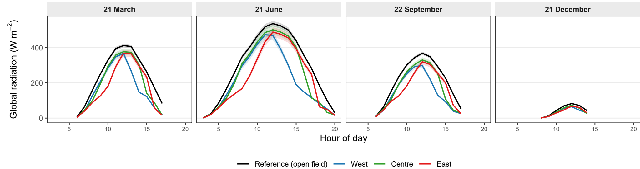
Simulated substrip global radiation on representative dates
