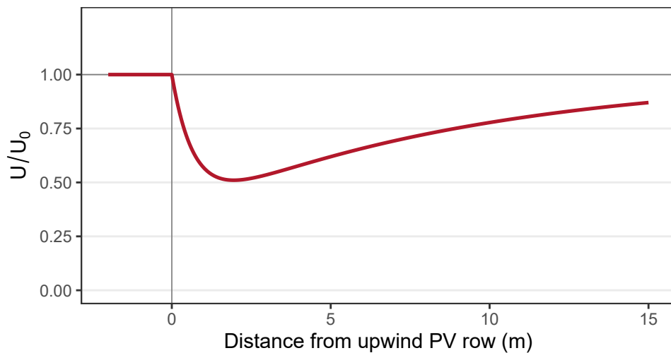
Barrier-profile reduction ( \beta_{APV} \approx 0.14 )
