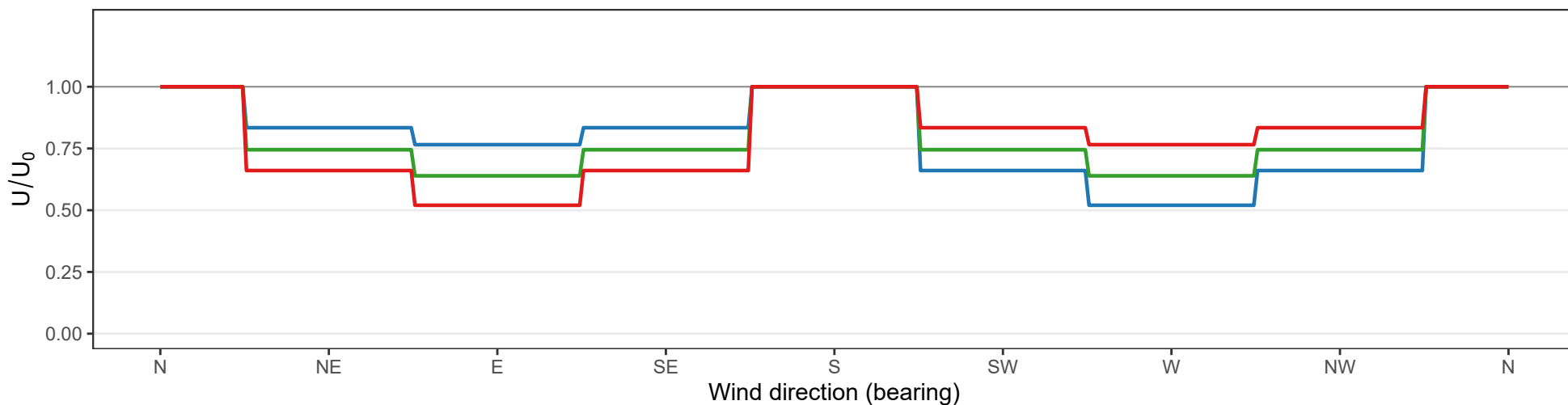
Direction-aware sheltering by substrip position
