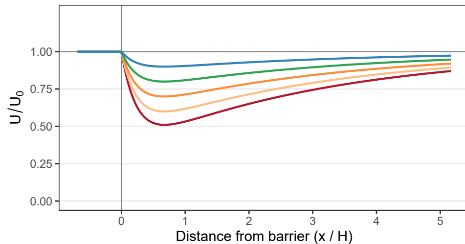
Sensitivity to panel porosity
