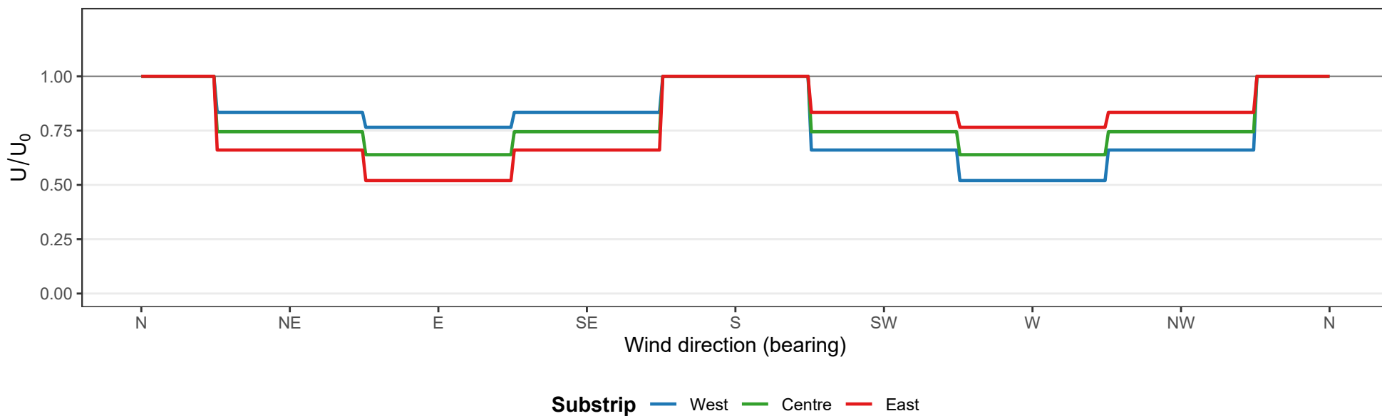
Direction-aware sheltering by substrip position
