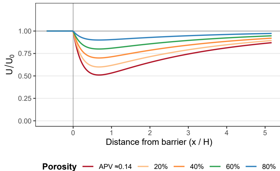
Sensitivity to panel porosity
