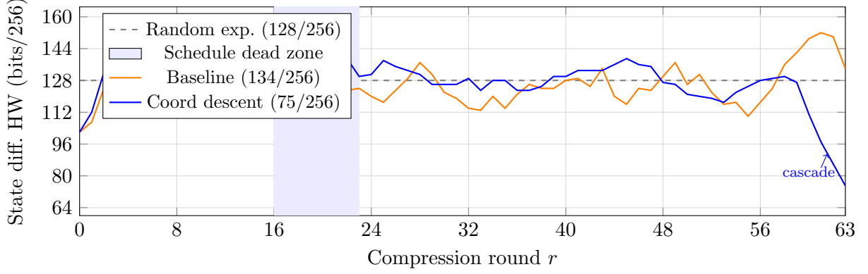
Figure 1: Round-by-round state differential HW for two block-2 messages sharing the Nine-Step IV (H_1, H'_1) . The shaded band marks the algebraic dead zone (schedule difference = 0, rounds 16–23). The coord-descent message exploits a suppression cascade in rounds 59–62, dropping from 127 to 75 bits.
