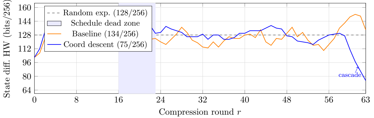
Figure 1: Round-by-round state differential HW for two block-2 messages sharing the Nine-Step IV ( H_1, H'_1 ). The shaded band marks the algebraic dead zone (schedule difference = 0, rounds 16–23). The coord-descent message exploits a suppression cascade in rounds 59–62, dropping from 127 to 75 bits.
