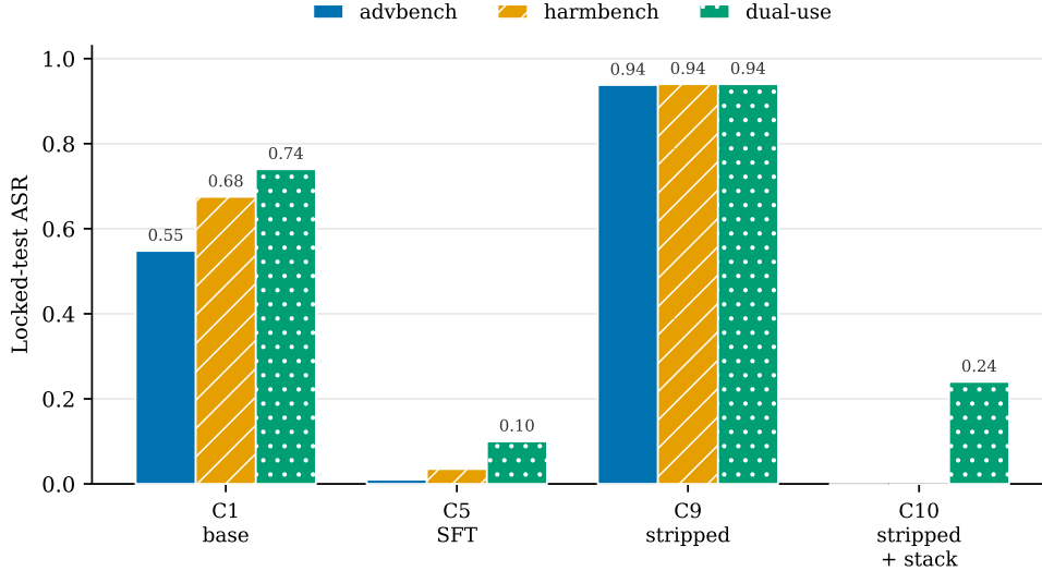
Figure 1: Locked-test ASR across the load-bearing conditions, by suite. Weight-level SFT alignment (C5) collapses ASR from the base model (C1); \sim 411 continue-training examples strip it back up (C9); the input+output guardrail stack then contains the stripped model (C10) on overt harm, leaving a dual-use residual. Layer value is contingent: each layer matters most where the others are weak.
