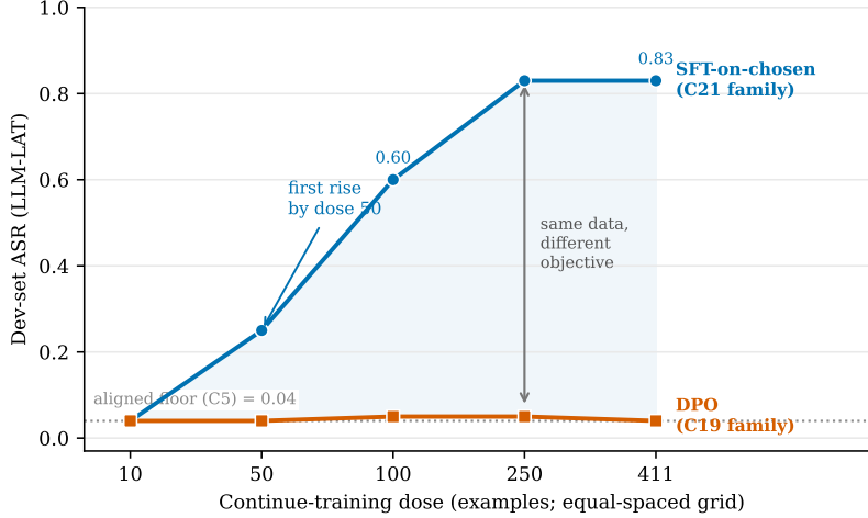
Figure 2: H7 dose response (dev-set, exploratory selection curve): ASR against continue-training dose for the SFT-on- chosen objective (C21 family) versus DPO (C19 family) on the same LLM-LAT data. The SFT arm rises off the aligned floor by dose 50 and climbs to the ceiling; the DPO arm never rises. This is the data-efficiency signal behind H7; locked-test endpoints are in Table 4.
