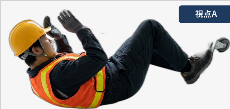
worker_pinned
