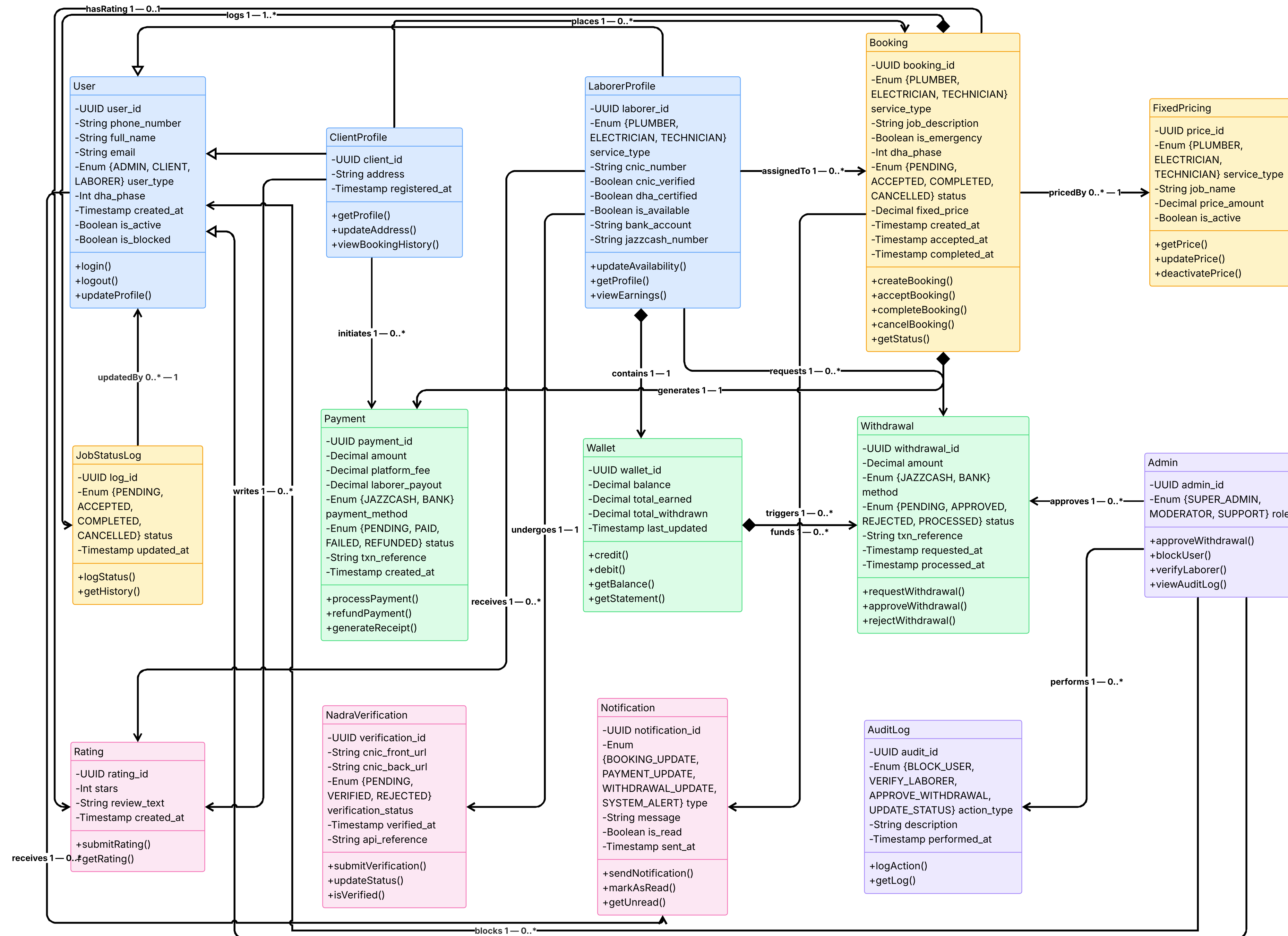
Figure 5. Karigar - Class Diagram
