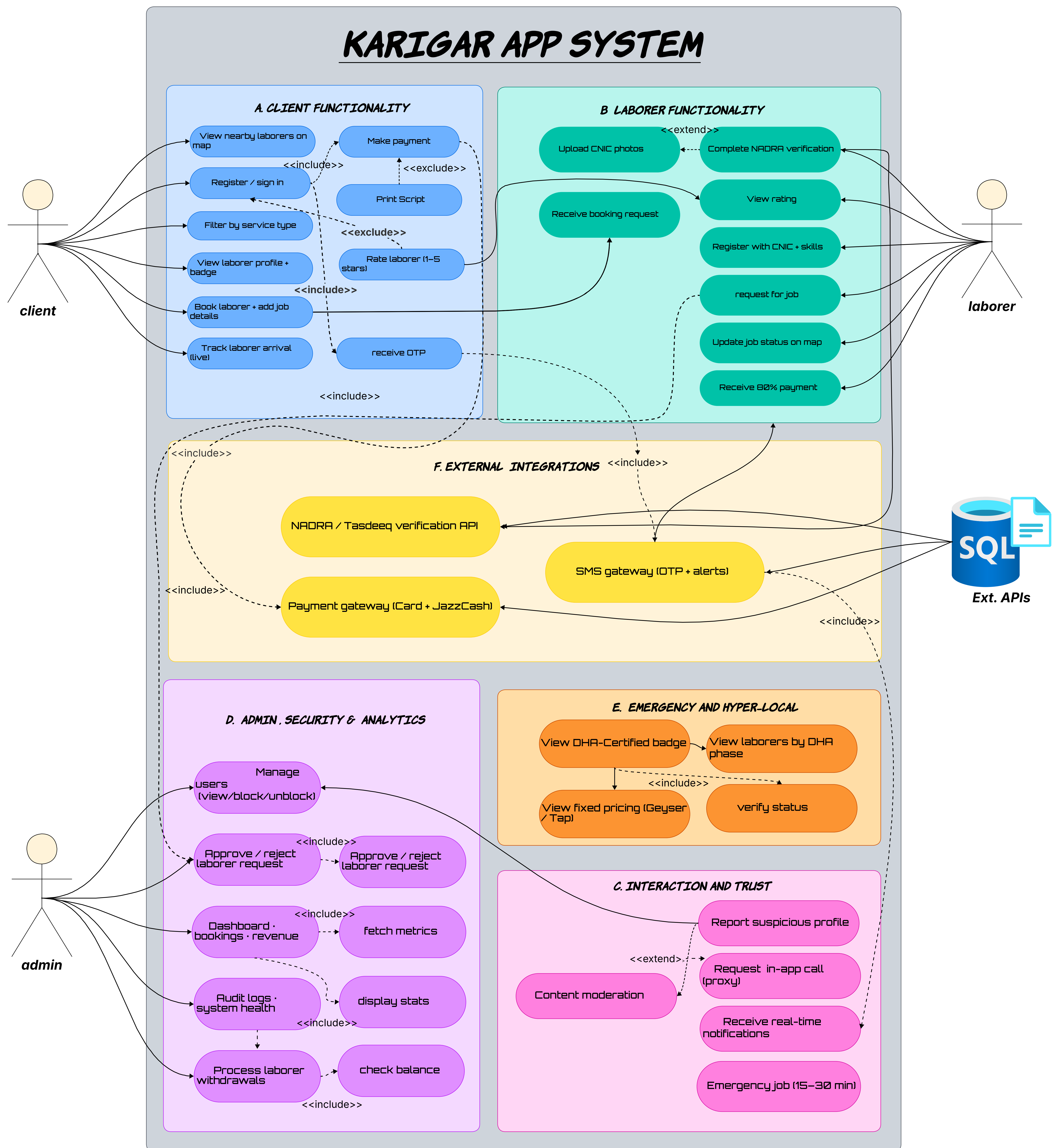
Figure 1. Karigar - Use Case Diagram
