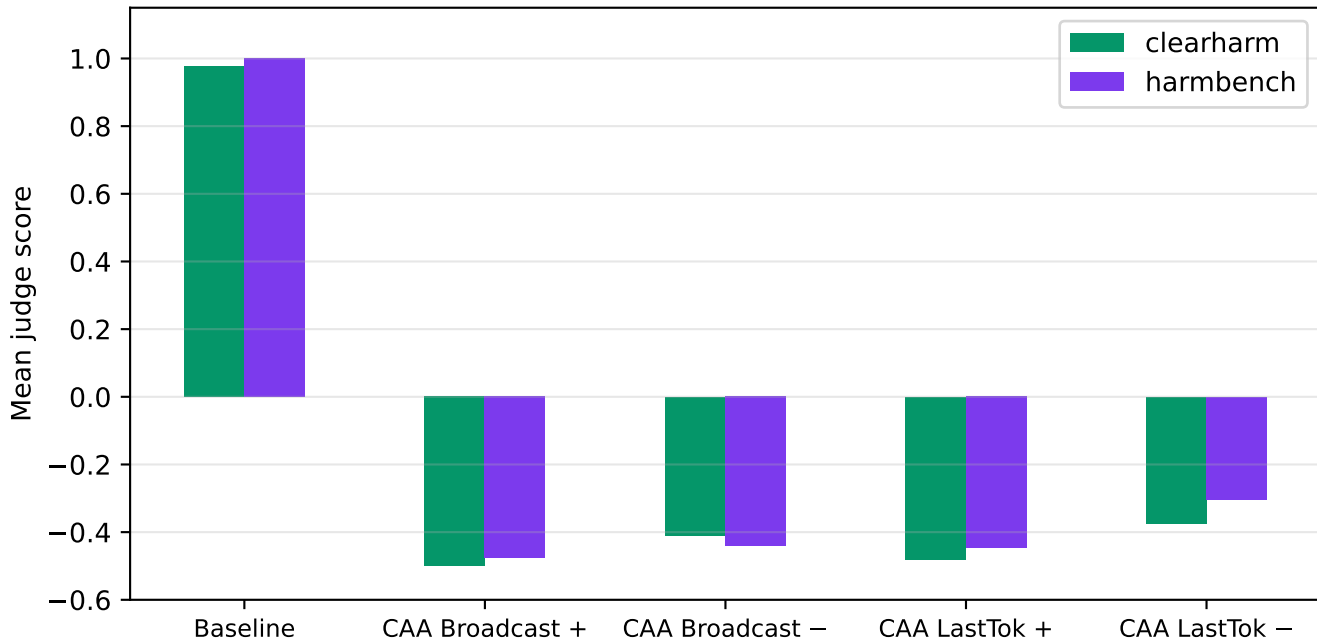
gemma-2-9b-it | safety | k=3.00 — by source
