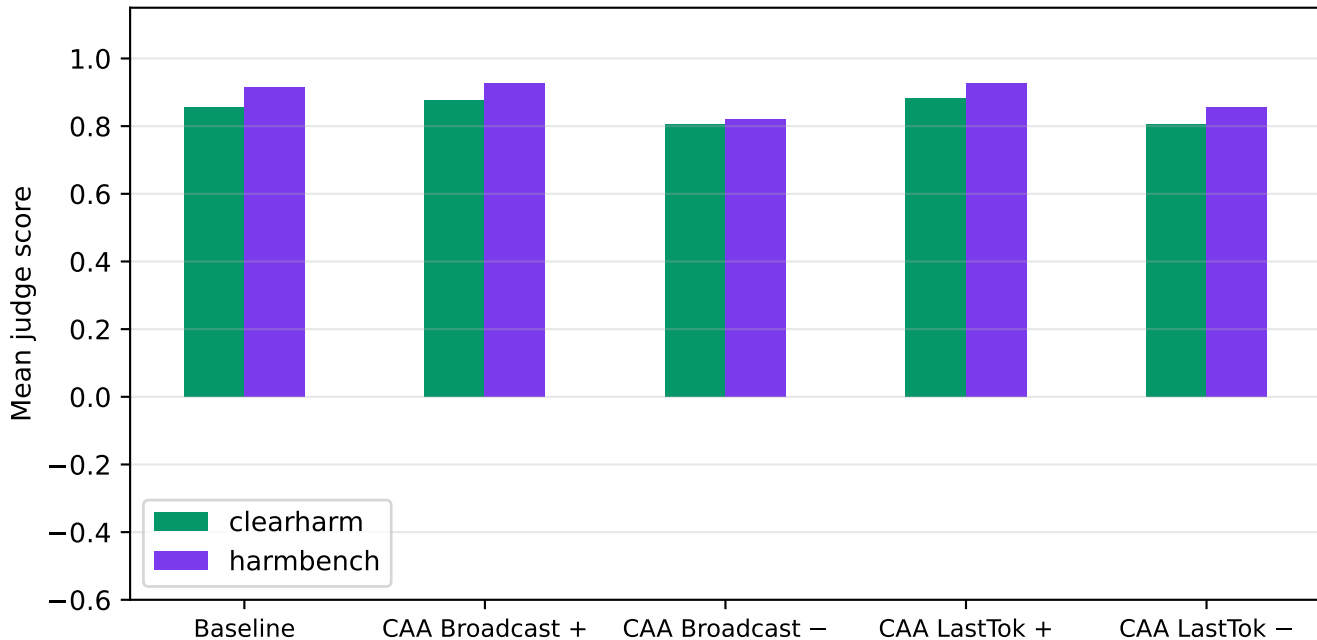
llama-3.1-8b-instruct | safety | k=0.50 — by source
