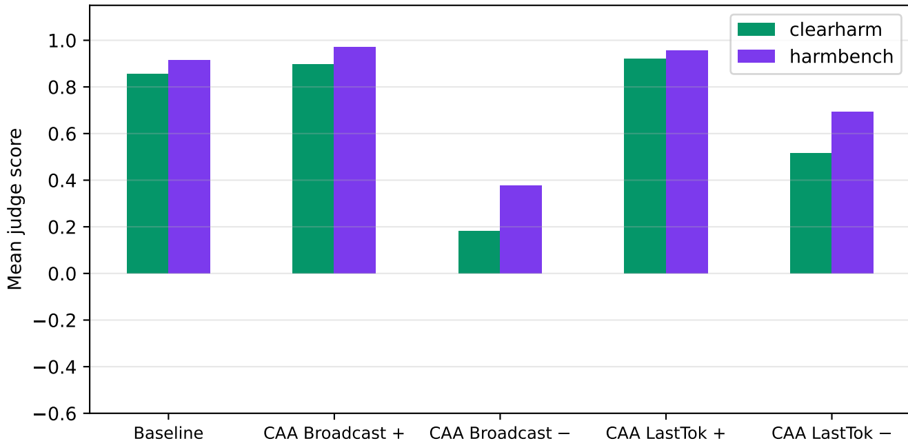
llama-3.1-8b-instruct | safety | k=2.00 — by source
