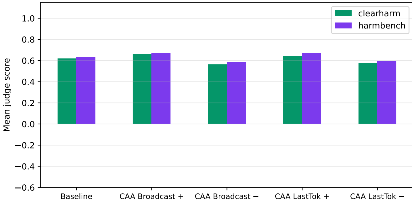
mistral-7b-instruct | safety | k=0.25 — by source
