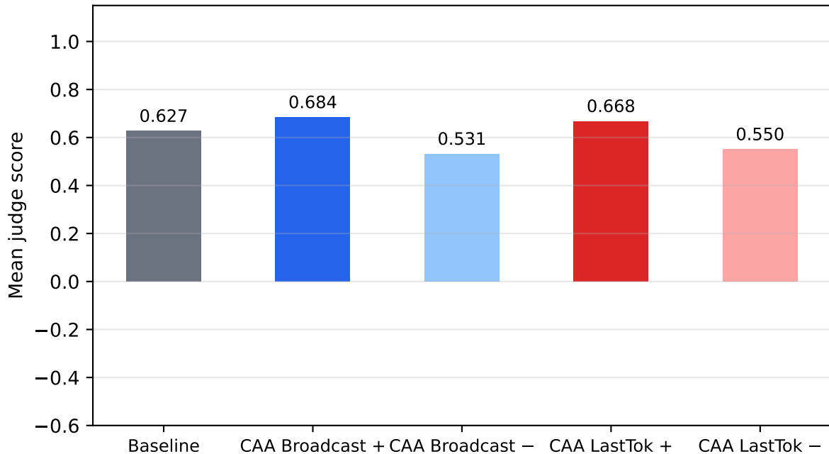
mistral-7b-instruct | safety | k=0.50
