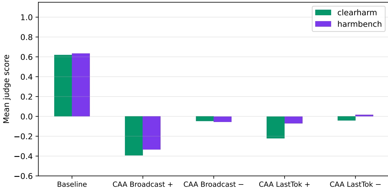
mistral-7b-instruct | safety | k=3.00 — by source
