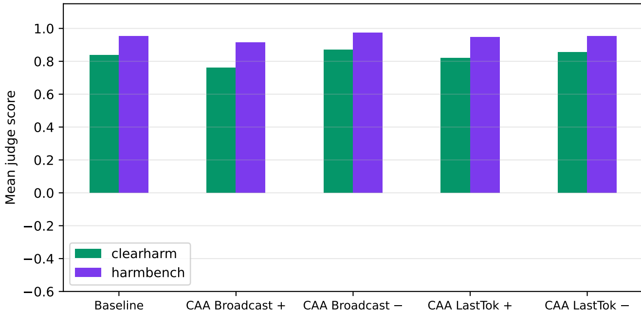
qwen2.5-7b-instruct | safety | k=0.25 — by source
