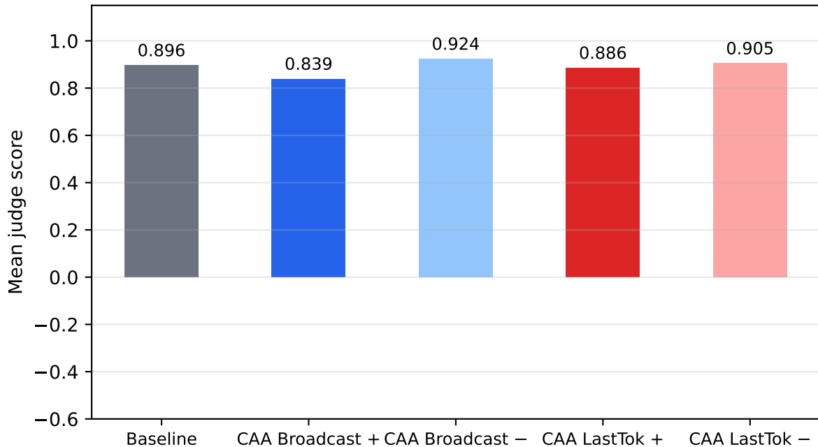
qwen2.5-7b-instruct | safety | k=0.25
