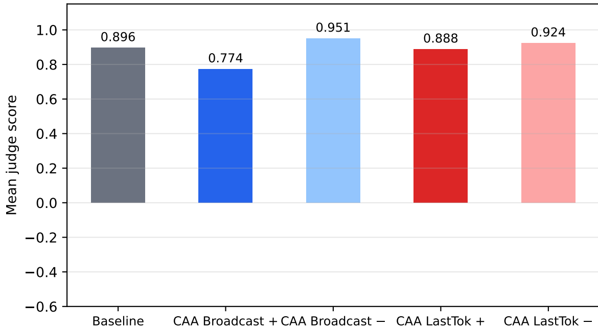
qwen2.5-7b-instruct | safety | k=0.50
