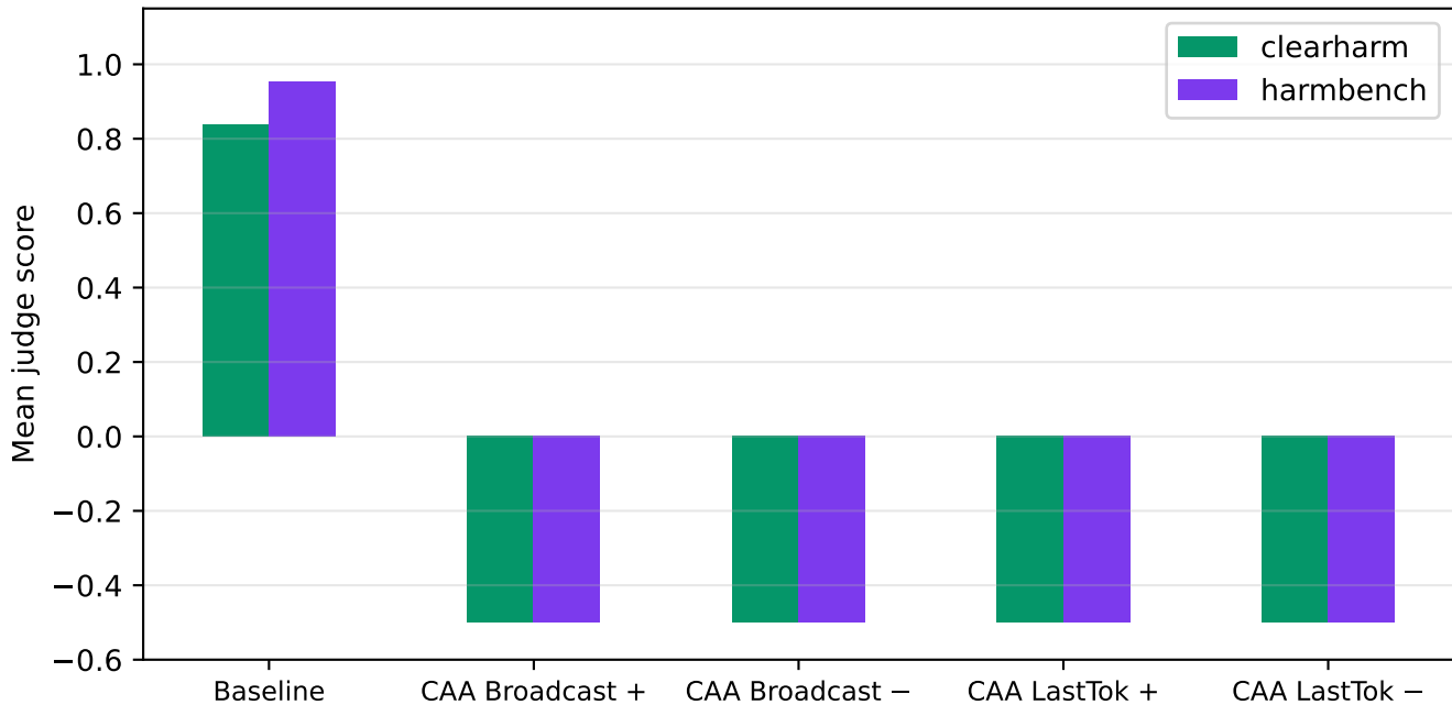
qwen2.5-7b-instruct | safety | k=5.00 — by source
