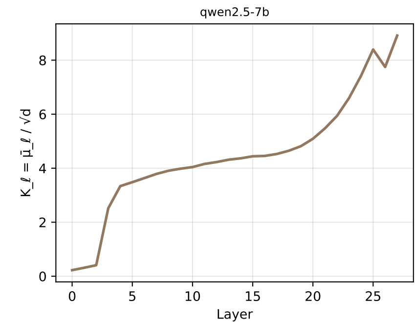
Calibrated K per layer ( K_l = \bar{\mu}_l / \sqrt{d} )
