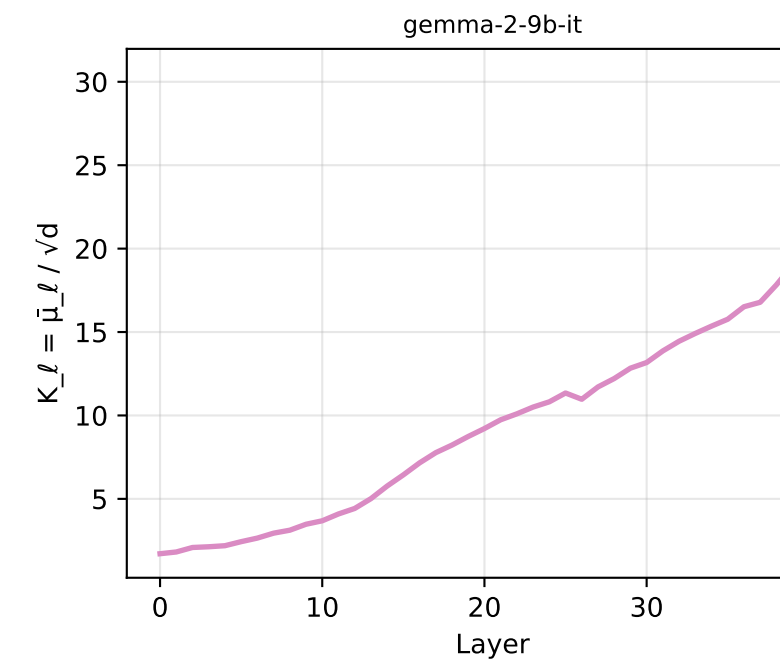
Calibrated K per layer ( K_l = \bar{\mu}_l / \sqrt{d} )
