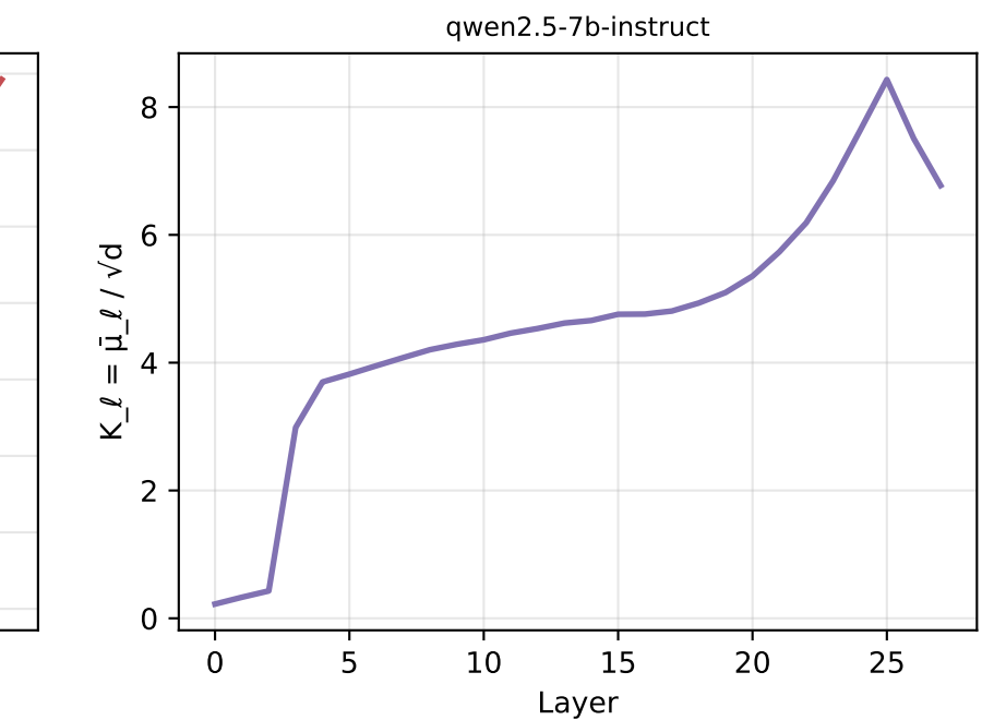
Calibrated K per layer ( K_l = \bar{\mu}_l / \sqrt{d} )
